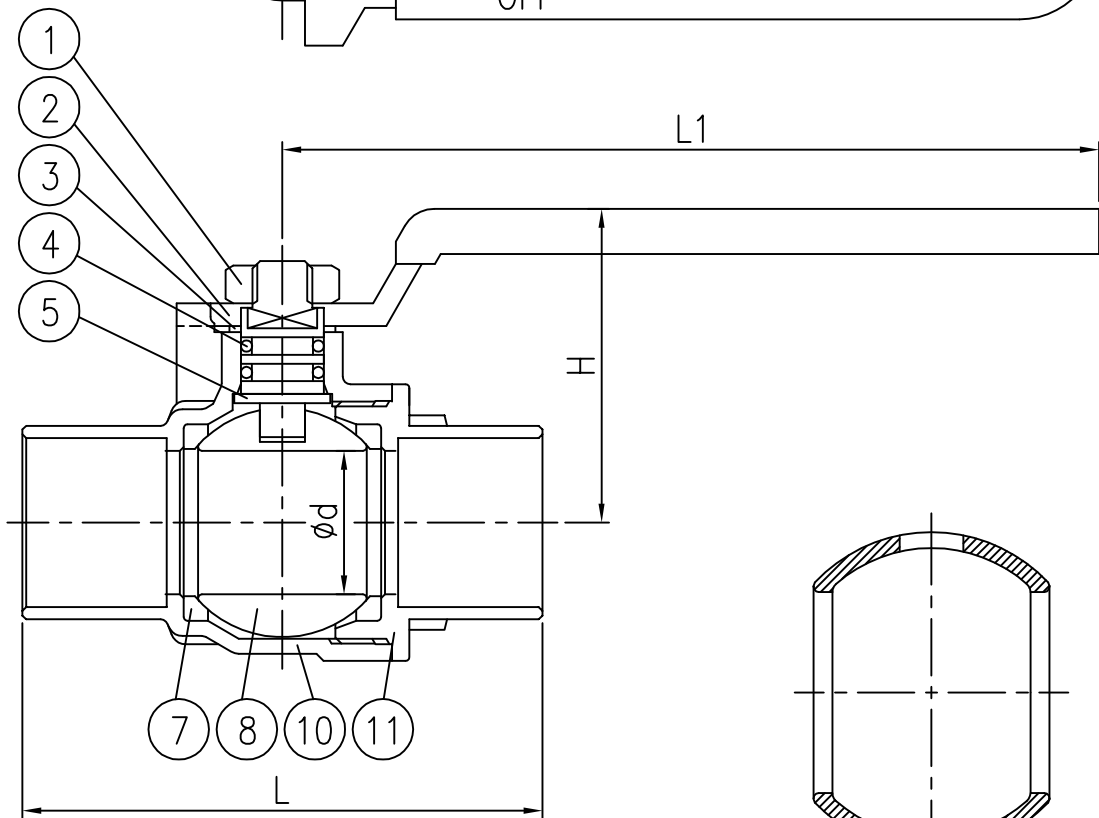
1"~3" BALL DISC
